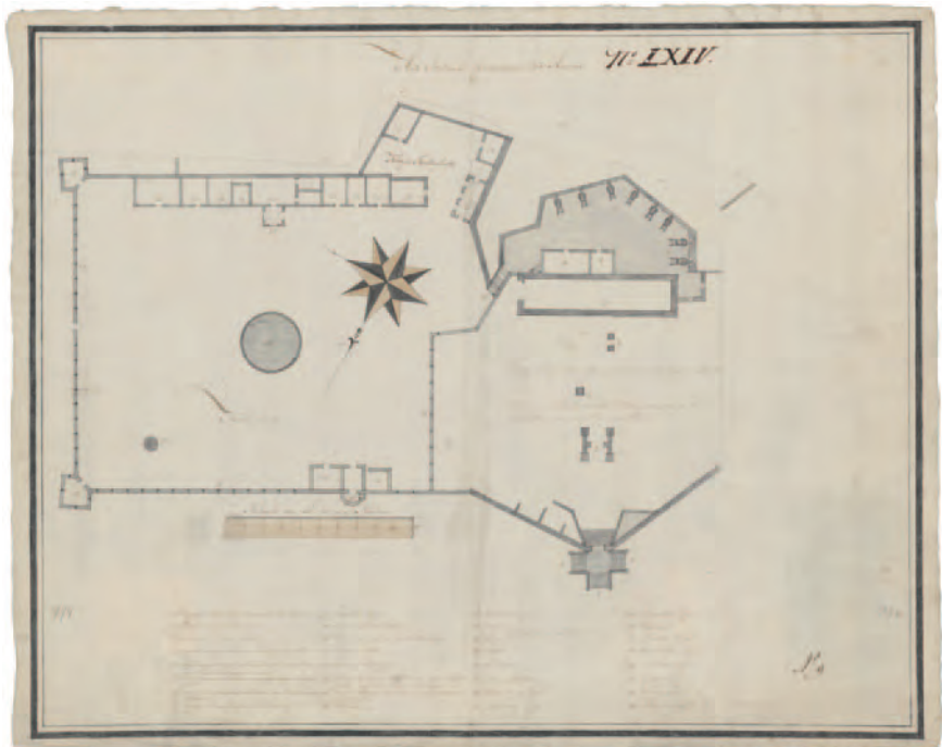
Plattegrond van Fort Crèvecoeur in Accra (Ghana), circa 1790.
